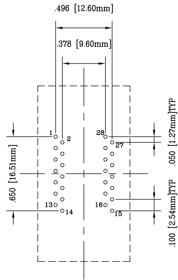
RECOMMENDED PCB LAYOUT AS SEEN FROM TOP OF SOCKET
