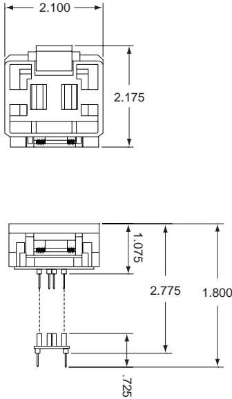
All Dimensions in Inches. (Assembly Drawing: (F5484))
