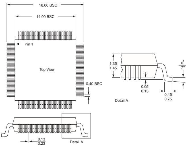
All Dimensions in Millimeters. ET CODE: 128-QF57D
