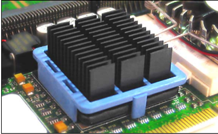
21MM Eliptical Fin BGA Heatsink w/ Clip
